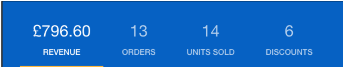
Store Dashboard
